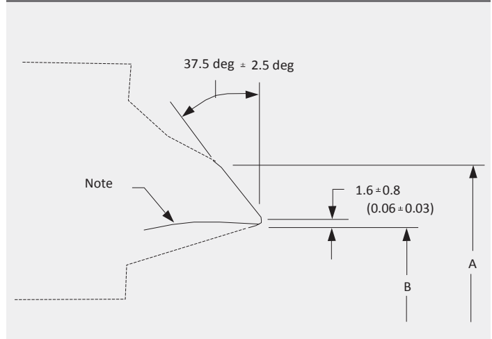
WELD BEVEL DETAIL FOR WALL THICKNESS OVER 22mm. (0,88in.)
